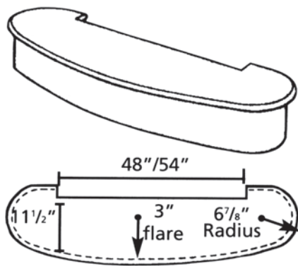
SW-8015B Bowed Starting Step Adjustable Oak
