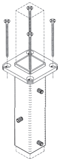
S-MB Metal Newel Fastener
